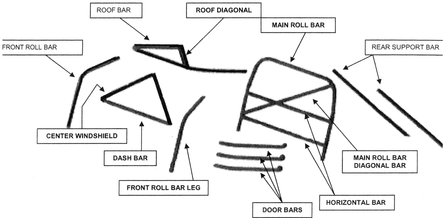
ROLL CAGE CONSTRUCTION DIAGRAM
